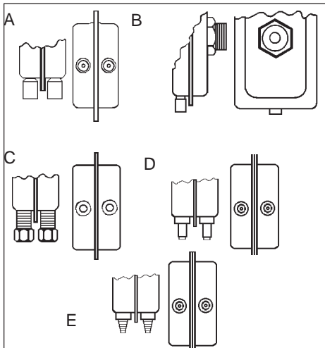
Figure 6. Typical Sample Line Connection Configurations for Series ANA Switches:
