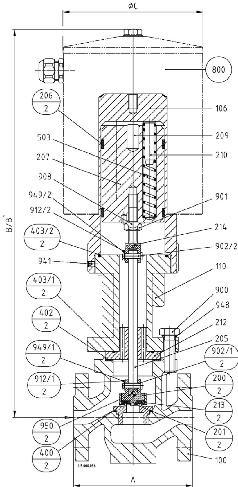
Fig.2 Flange design: 10/20-EVA
