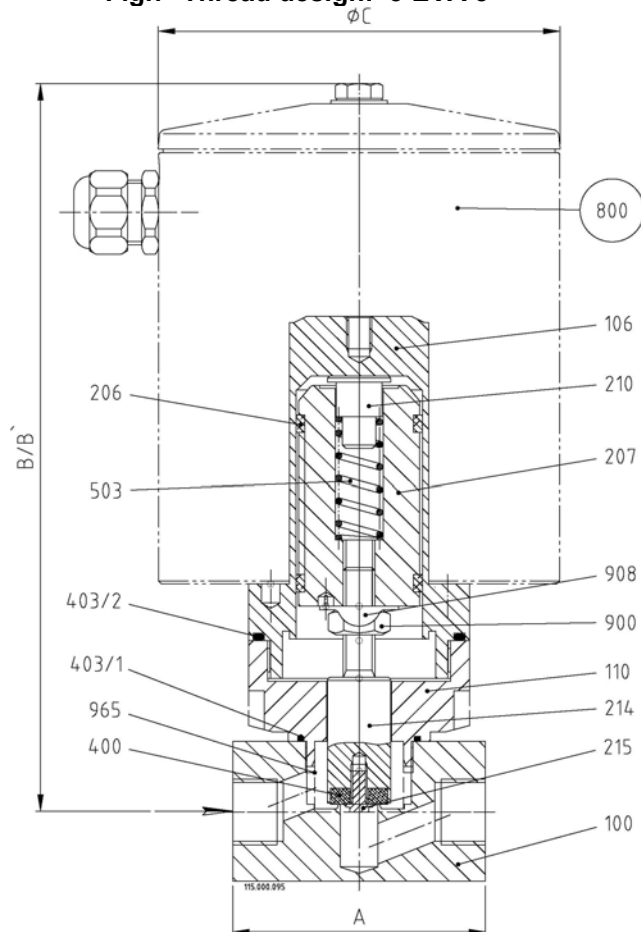
Fig.7 Thread design: 5-EVA 5
